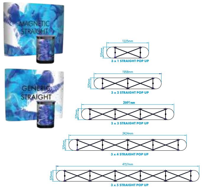
MAGNETIC/GENERIC POP-UP STRAIGHT POPM/G-S
