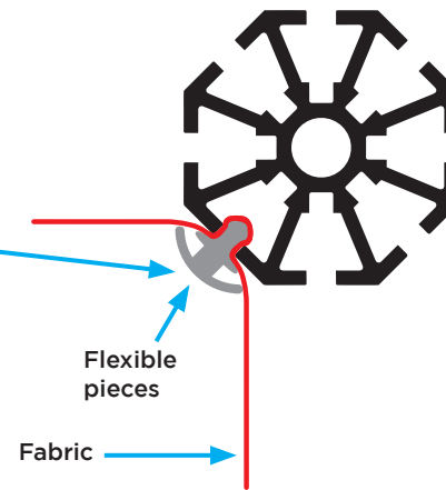
Shell scheme corner post seen from above
